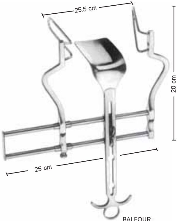
BALFOUR L 532.01 Yan Bleyd 105 mm Lateral Blades Orta Bleyd L 580.23 Center Blade 107 x 59 mm
